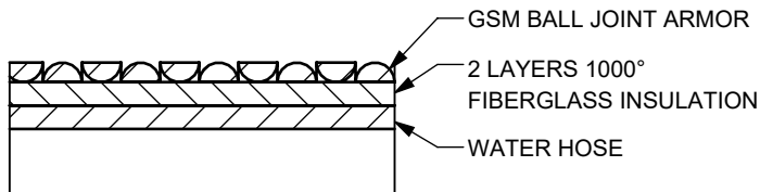
DETAIL A SCALE 3 : 4
