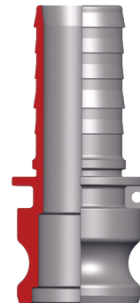
Type E adapter and hose shank
