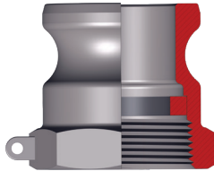
Type A adapter and female NPT
