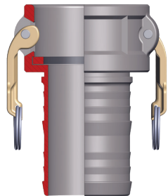
Type C coupler and hose shank
