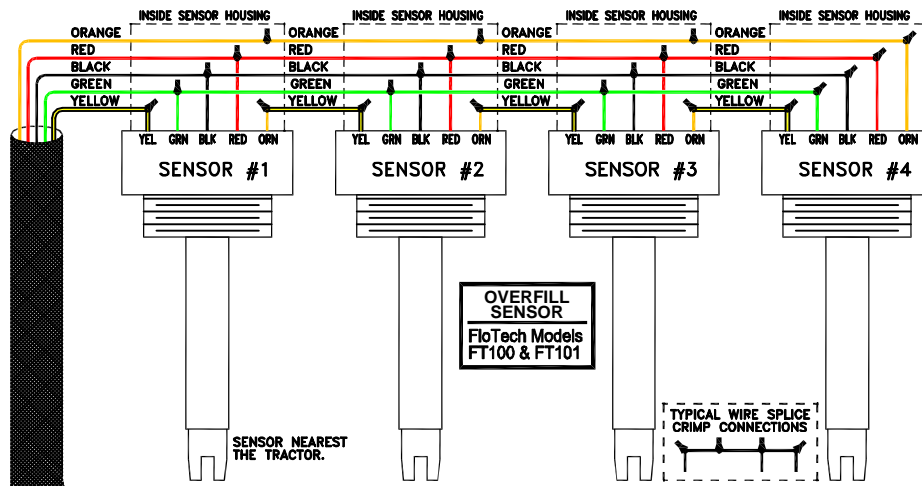
FloTech 5 wire cable. Model FT400
